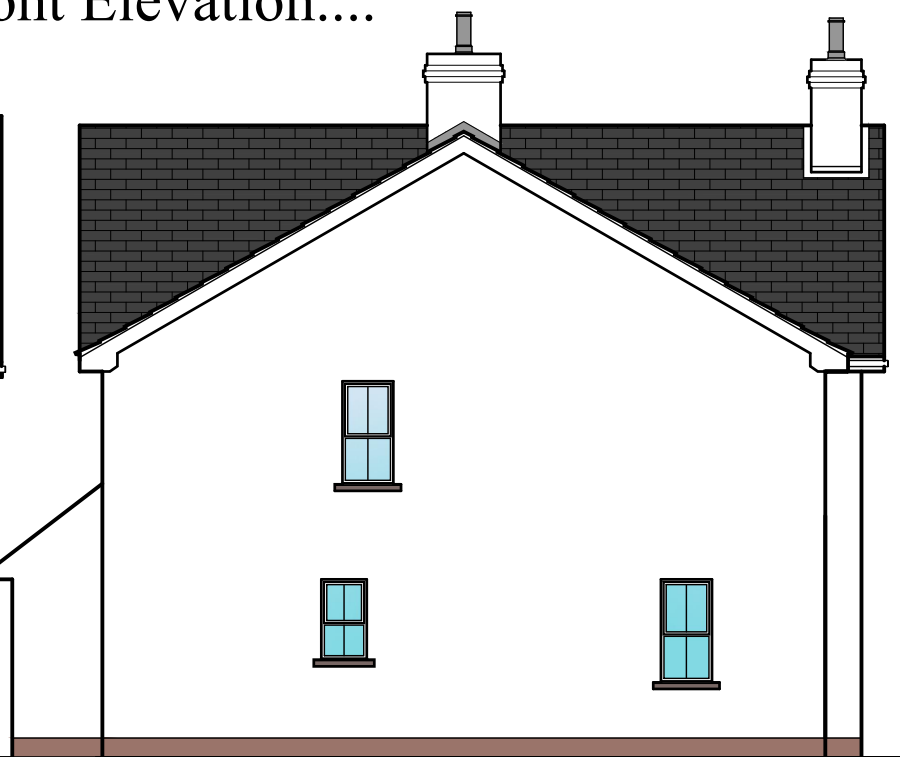
Side Elevation....
