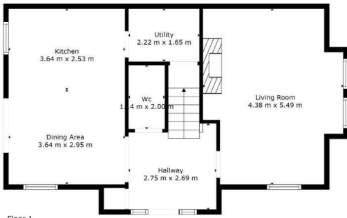
Floor 1
