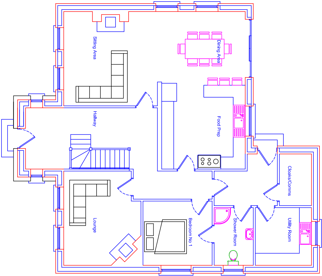
Ground Floorplan
