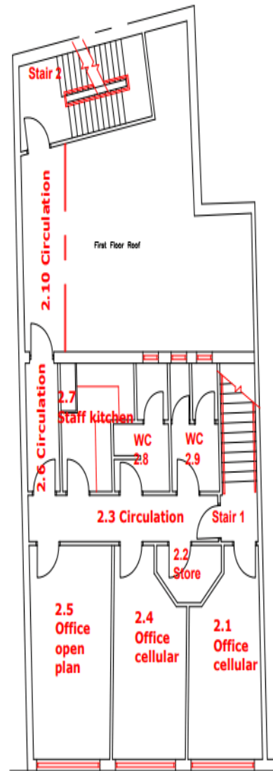
SECOND FLOOR
