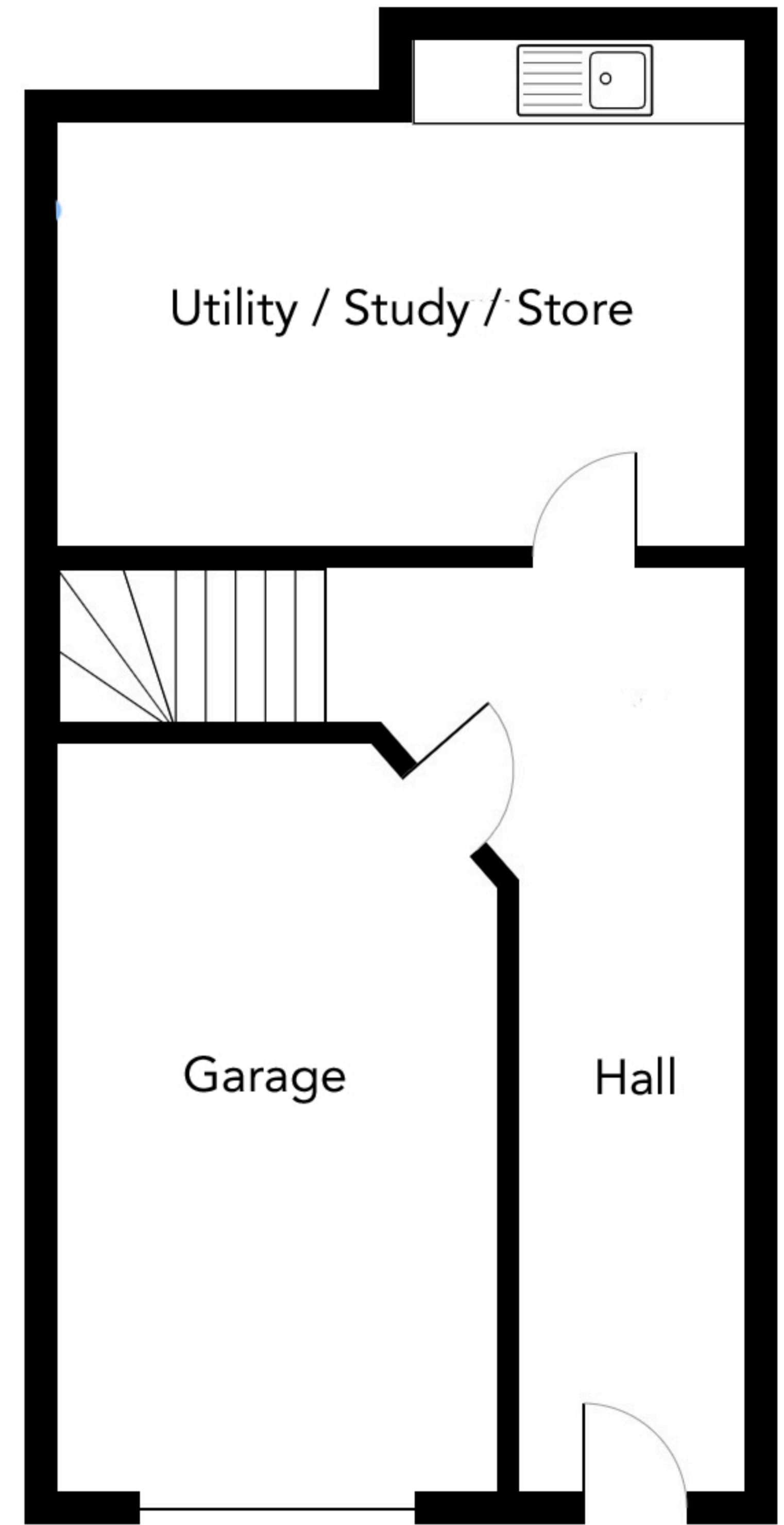
Ground Floor
