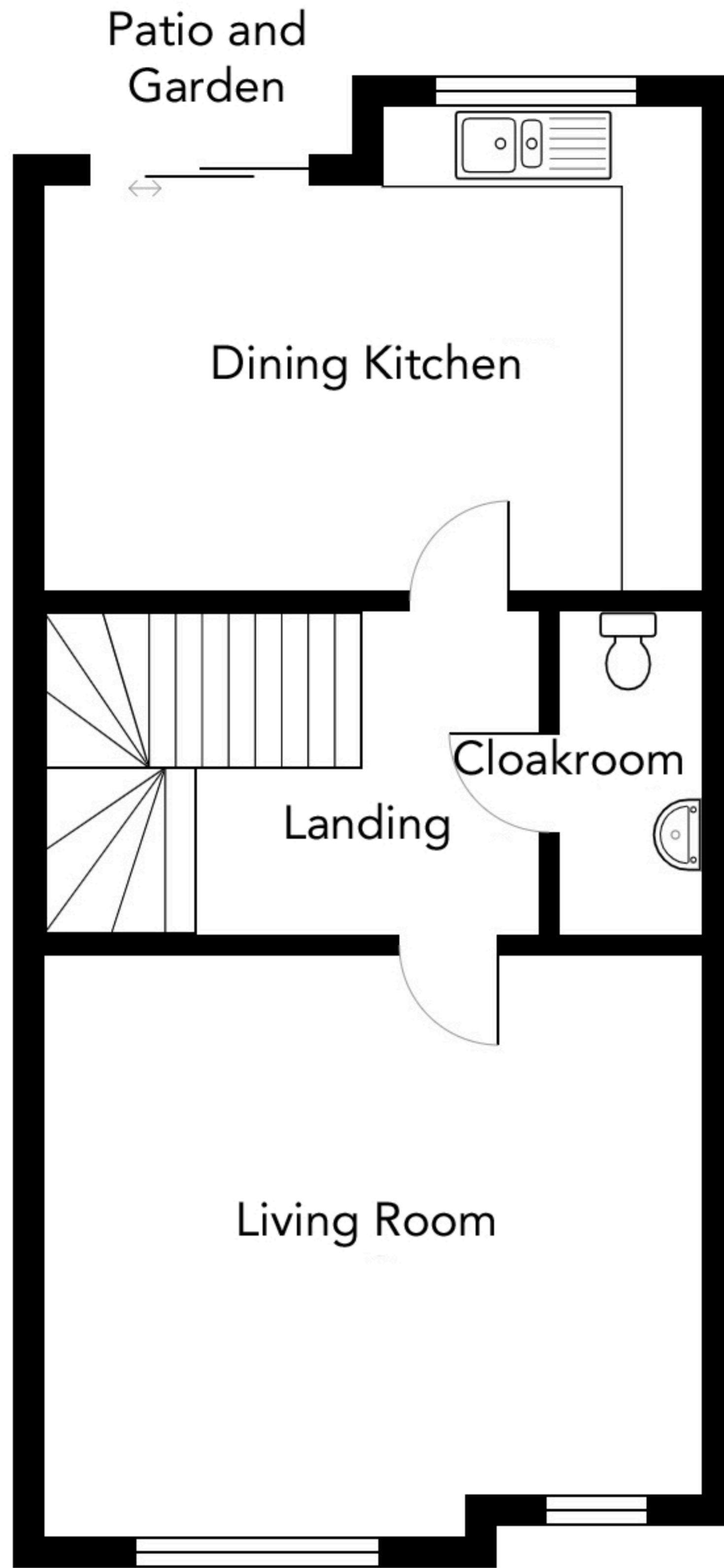
First Floor
