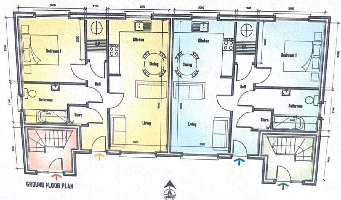
TYPE "C" - 1 Bedroom Apartment (Site Nos 8 - 11)
