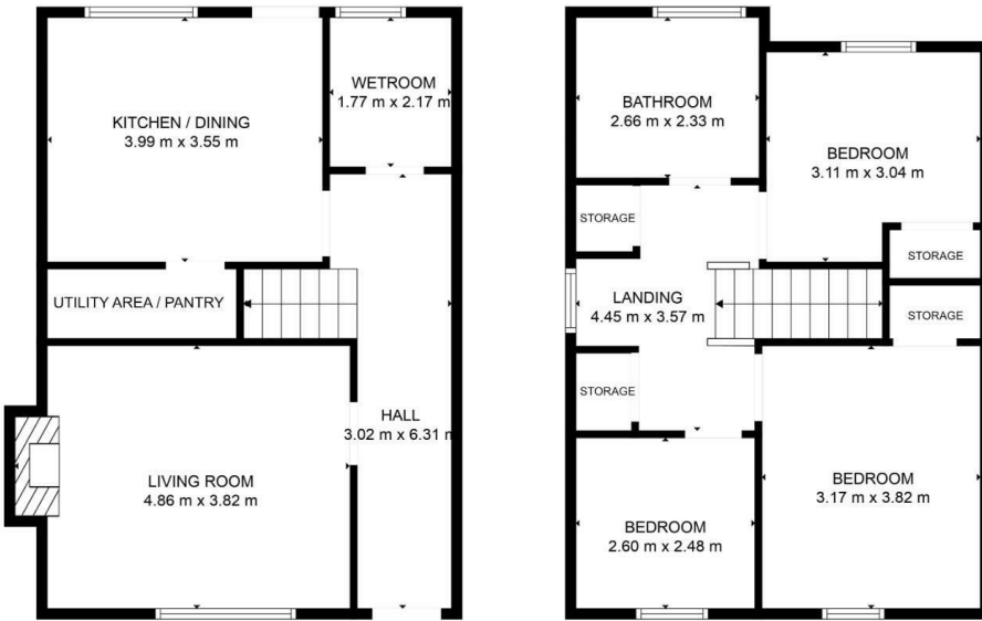
FLOOR 1
