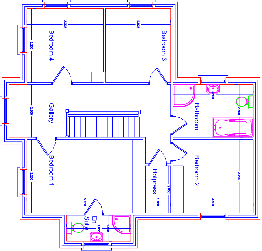
House Type E First Floorplan
