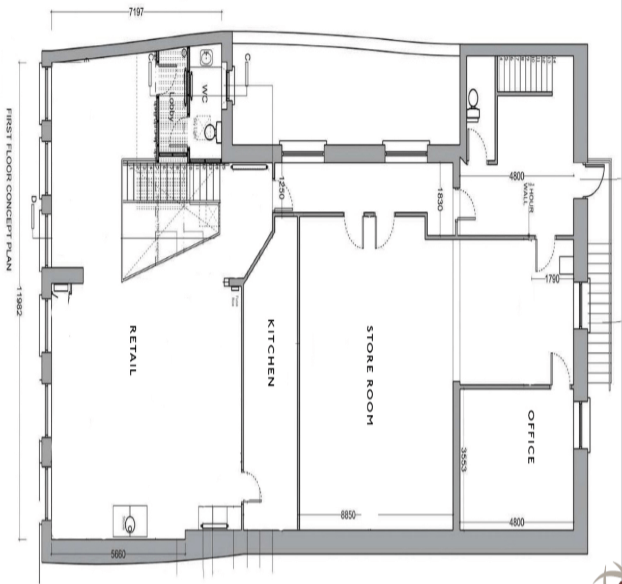
Indicative First Floor Plan
