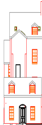
Proposed Elevation to Mews Lane
