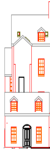
Proposed Elevation to Mews Lane
