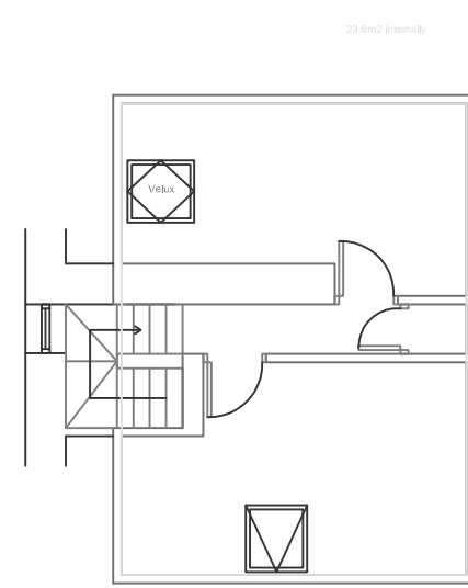
EXISTING SECOND FLOOR PLAN SCALE 1:50
