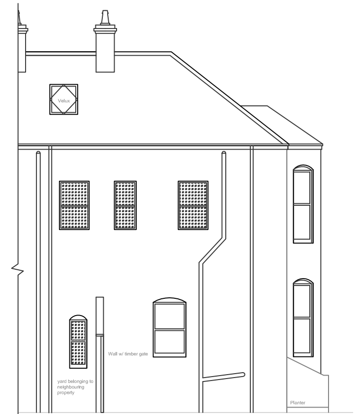
EXISTING SOUTH WEST ELEVATION SCALE 1:50
