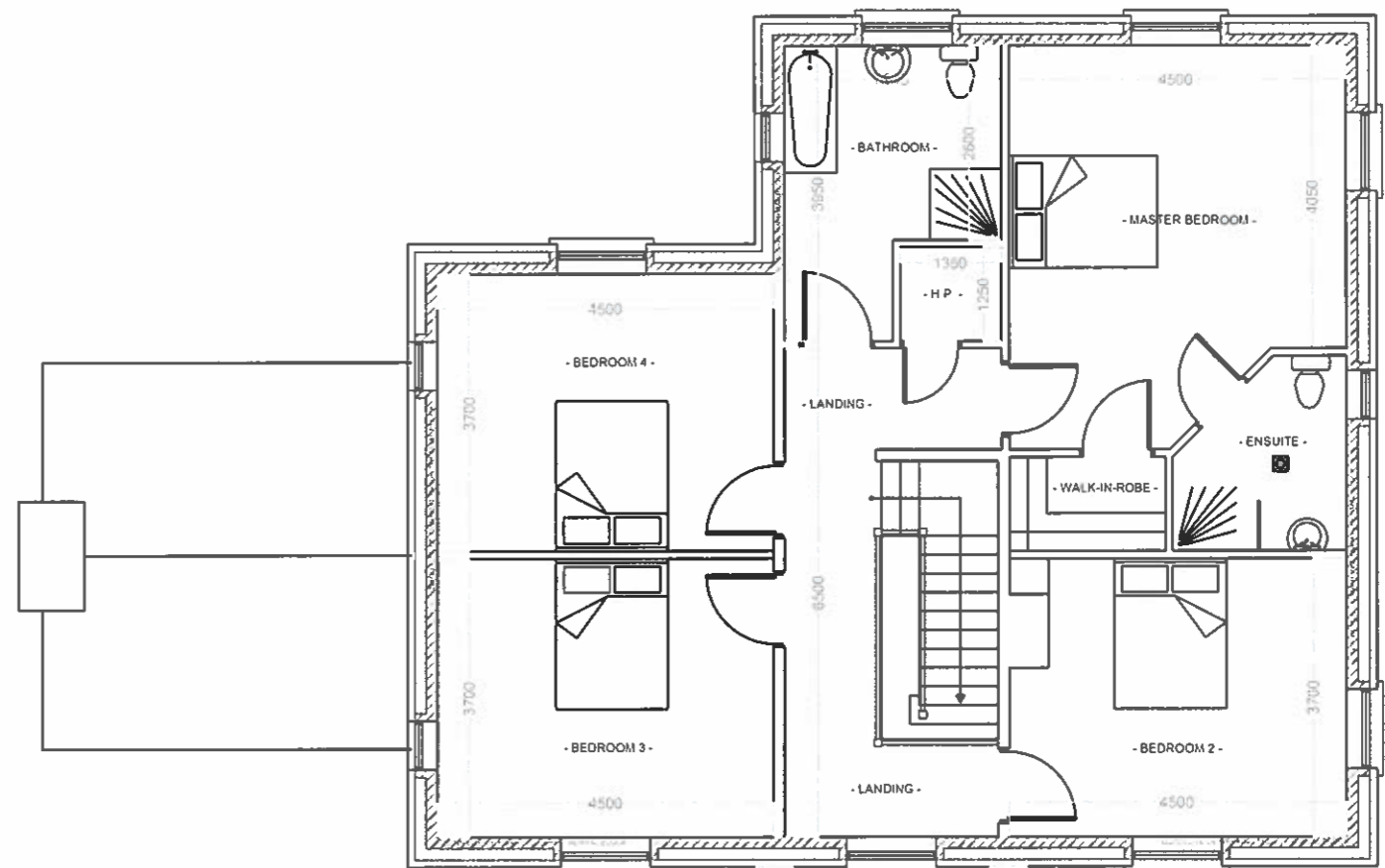
- PROPOSED FIRST FLOOR PLAN - 114m 2
