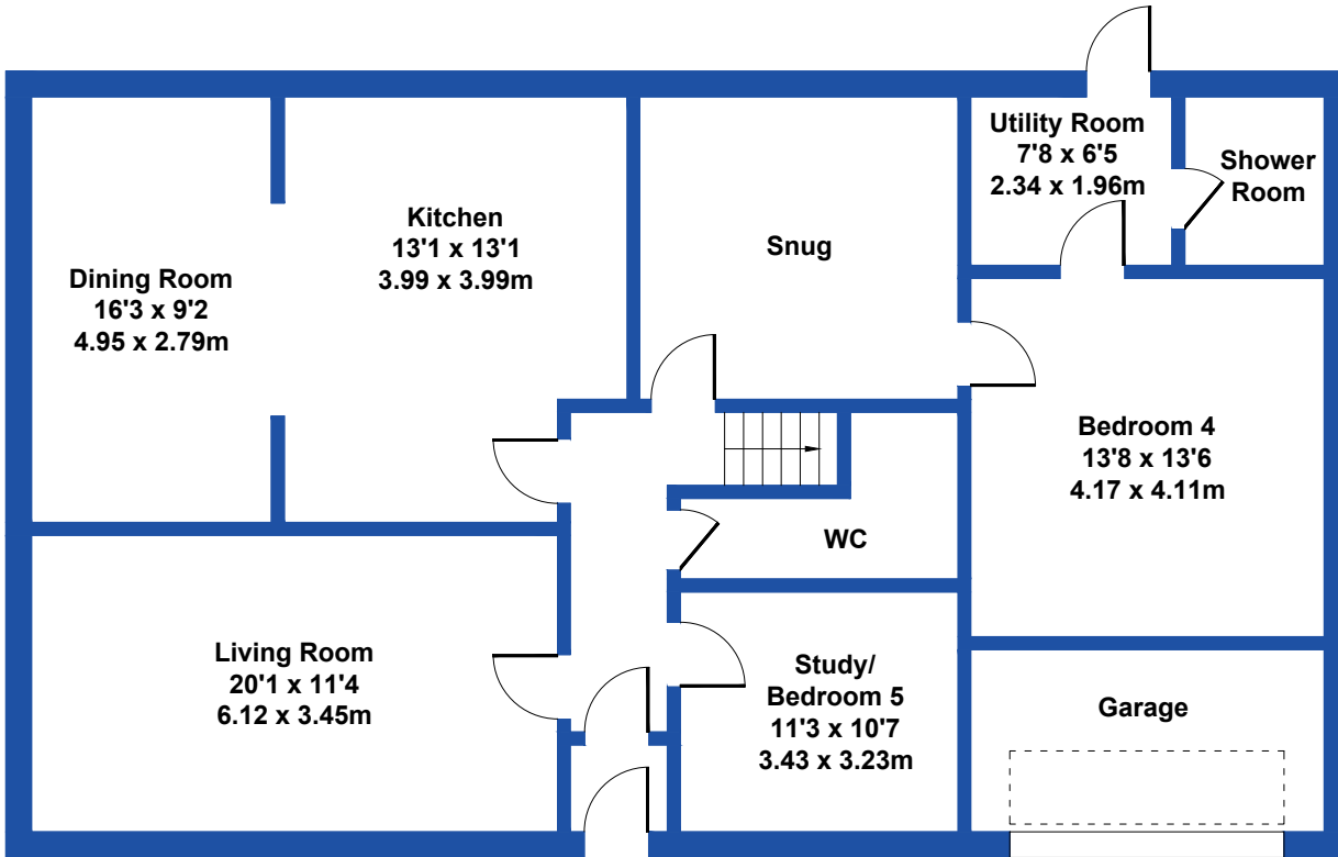
GROUND FLOOR
