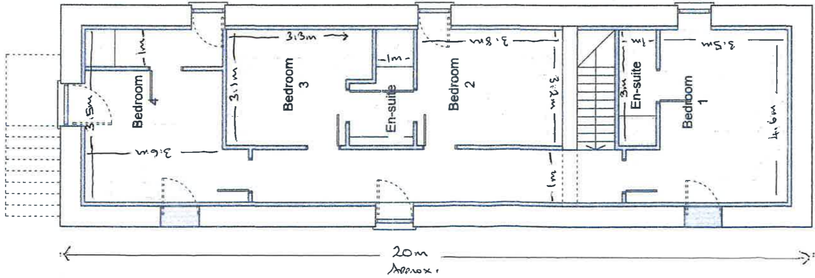
First Floor
