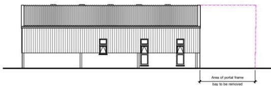
North Elevation 1:100
