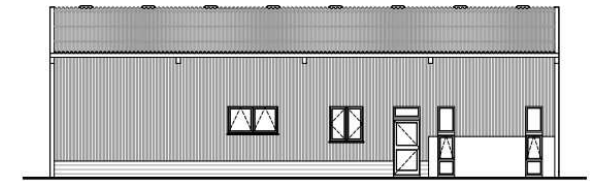
North Elevation 1:100
