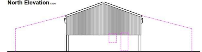
North Elevation 1:100
