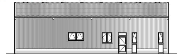
West Elevation 1:100
