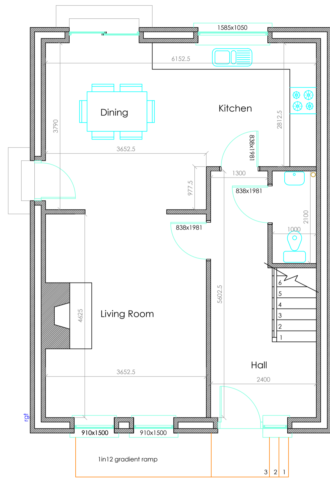
Ground Floor Plan CA4 Site 154
