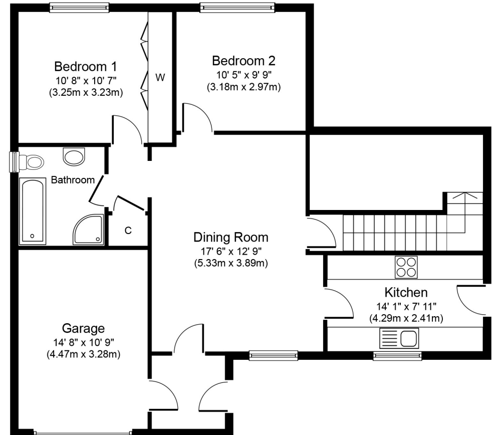
Ground Floor Approximate Floor Area 991 sq. ft. (92.1 sq. m.)
