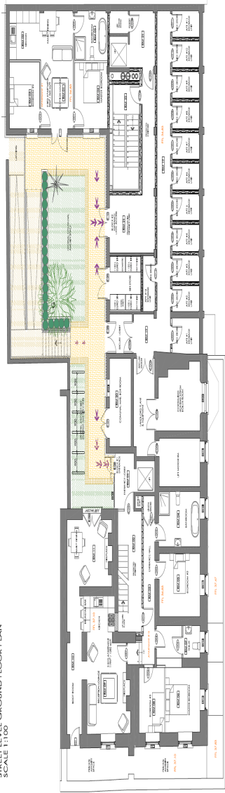
LOWER GROUND FLOOR (BASEMENT) PLAN SCALE 1:100
