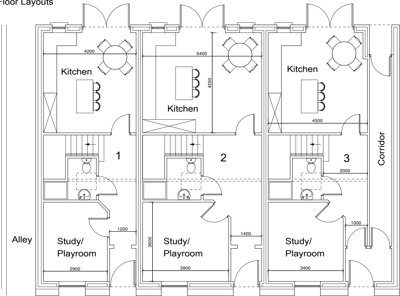
Ground Floor Layouts
