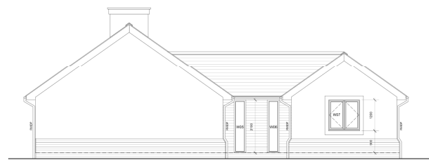
PROPOSED SIDE ELEVATION Plot 38 Scale 1:50
