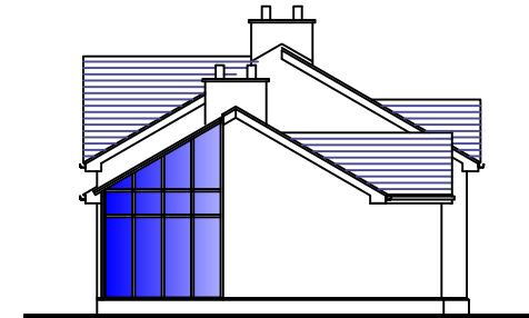
EAST ELEVATION
