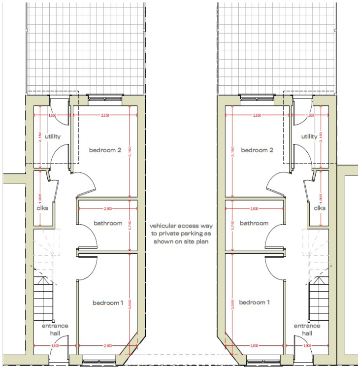
Ground Floor as Proposed
