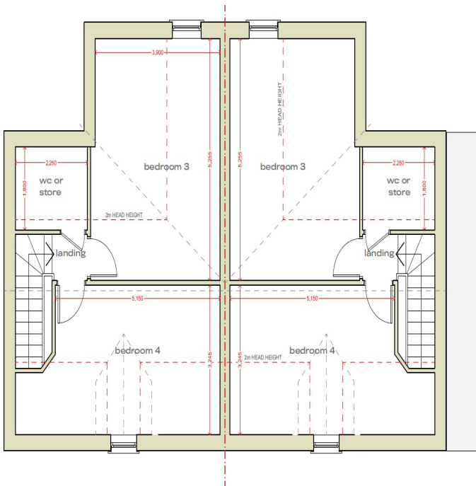
Second Floor as Proposed
