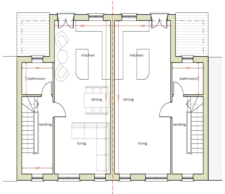
First Floor as Proposed
