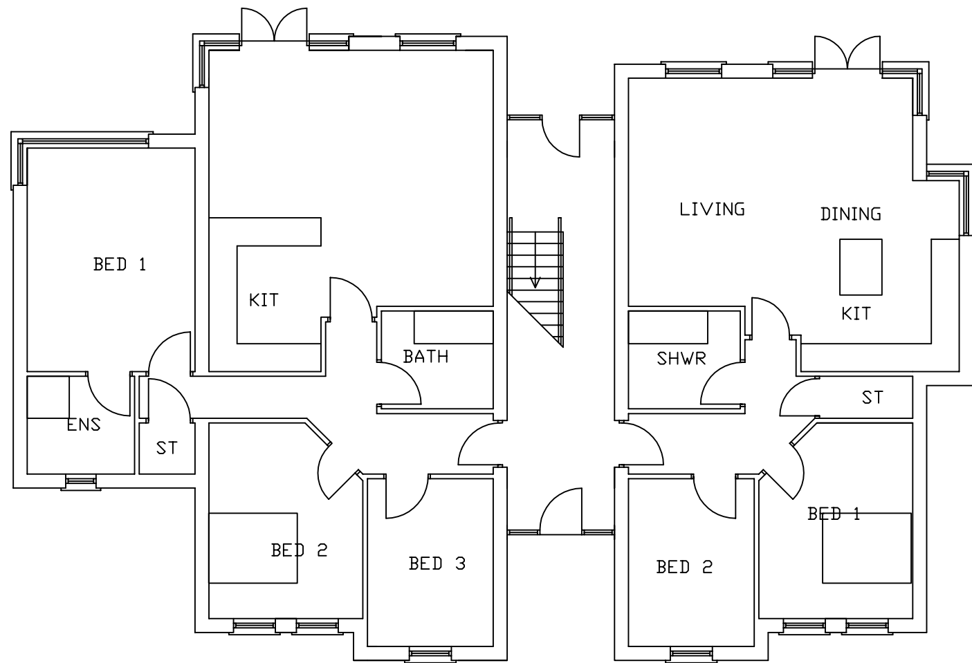
GROUND FLOOR PLAN ( BLOCK A )
