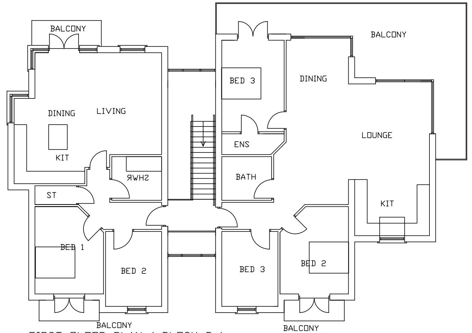
FIRST FLOOR PLAN ( BLOCK B )
