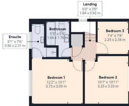
Floor 1
