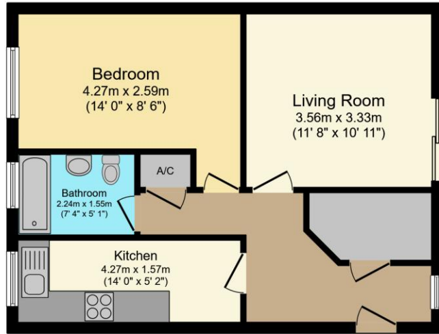
Floor Plan Floor area 46.9 sq.m. (504 sq.ft.)
