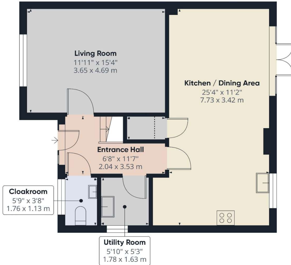
Floor 0 Building 1
