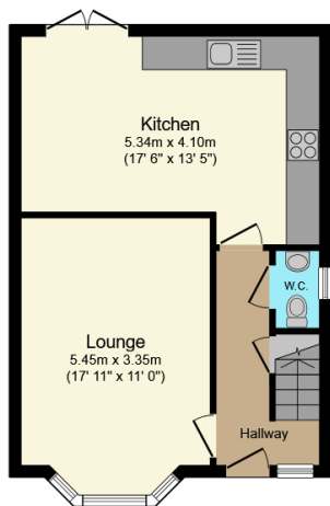
Ground Floor Floor area 42.5 m 2 (457 sq.ft.)
