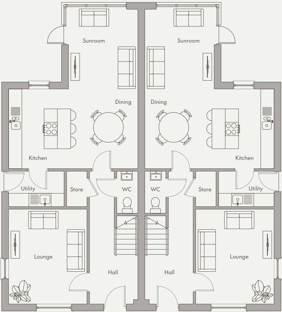
Ground floor
