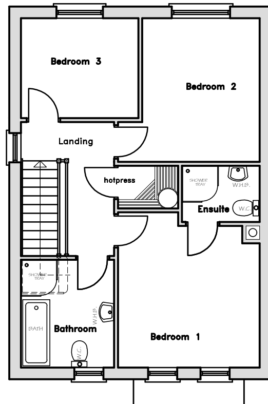
FIRST FLOOR PLAN Scale - 1:50
