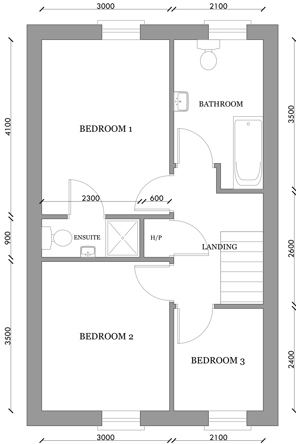
FIRST FLOORPLAN
