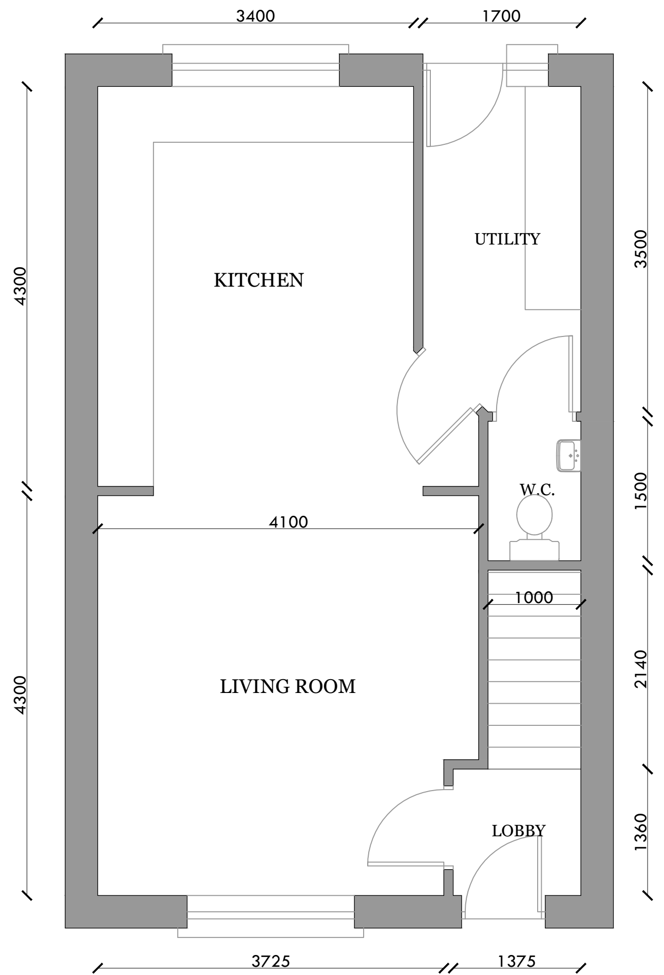
GROUND FLOORPLAN
