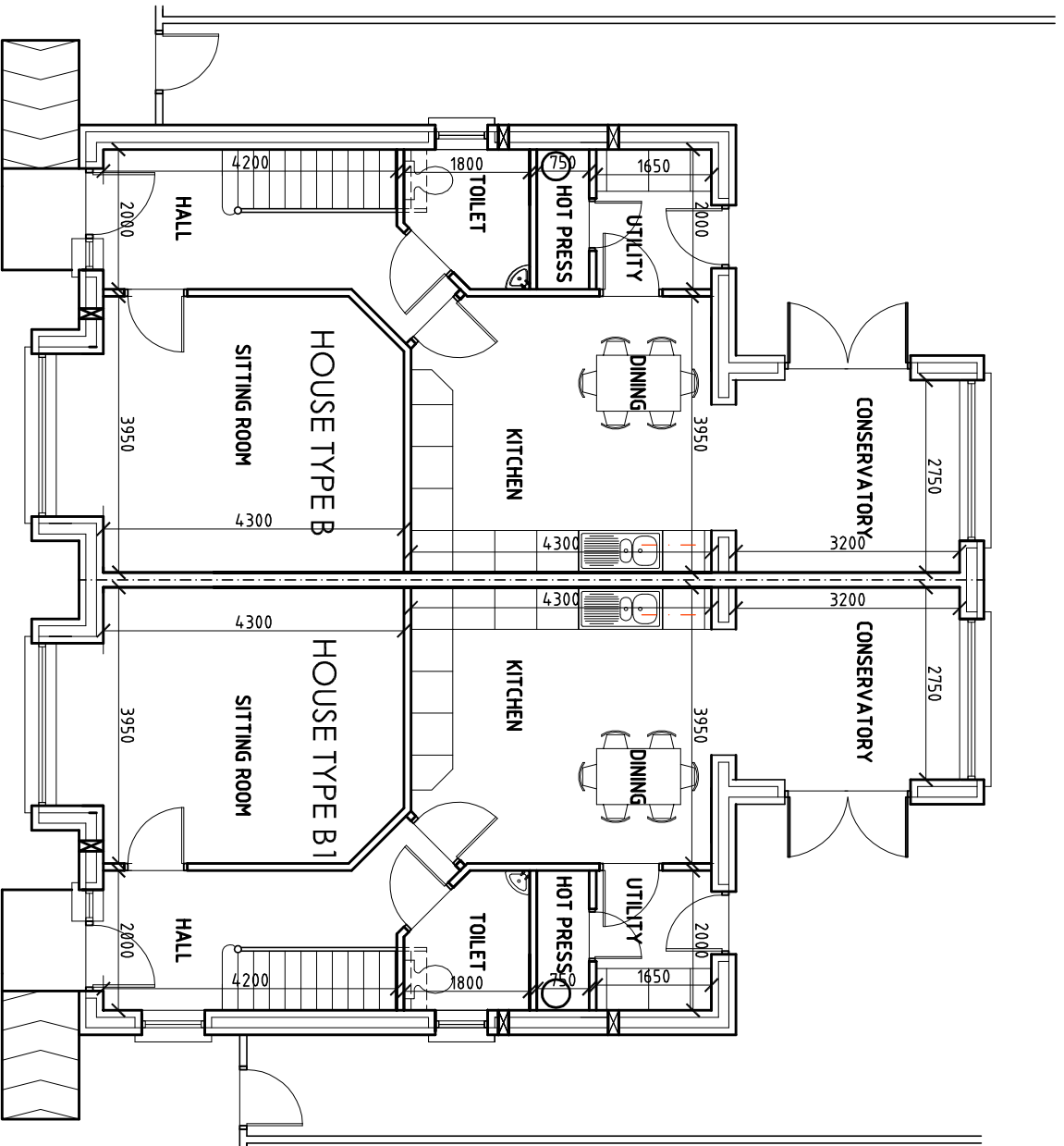
HOUSE TYPE B 3-bed GROUND FLOOR PLAN Area = 63.98 sq.m. (incl. conservatory) Total Floor Area = 118.18 sq.m.
