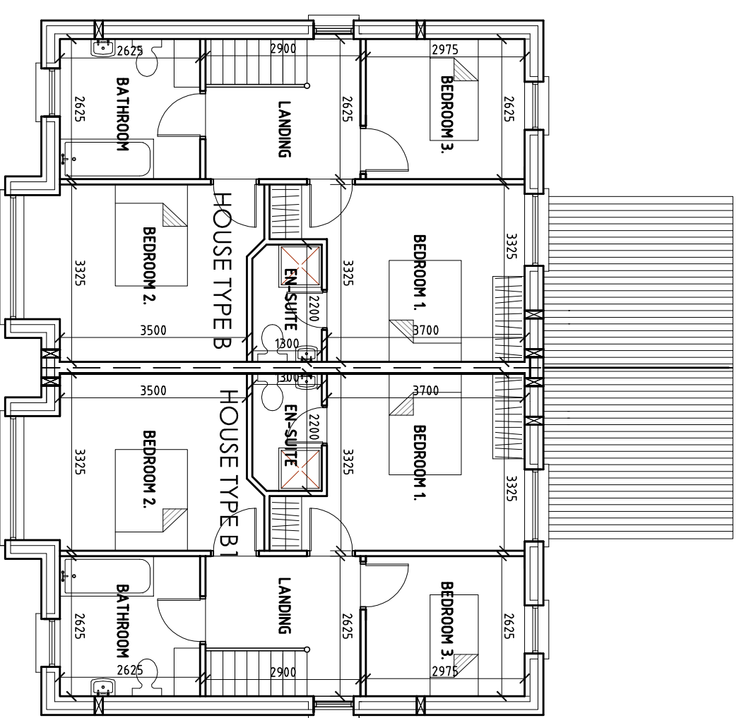
HOUSE TYPE B 3-BED FIRST FLOOR PLAN Area = 54.20sq.m.
