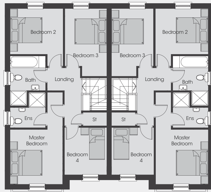
First Floor
