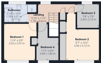
Floor 1
