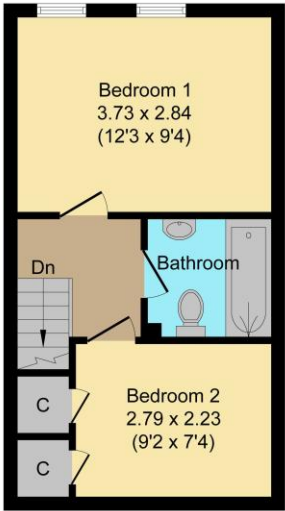
First Floor Floor area 25.90 sq.m. (278.78 sq.ft.)
