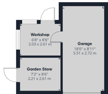
Floor 0 Building 3
