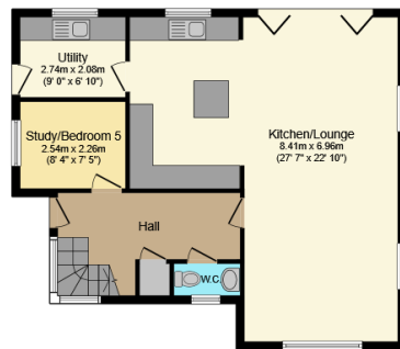
Ground Floor Floor area 72.8 sq.m. (783 sq.ft.)
